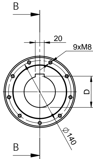
27001009700 - W-Boss/14216070G7/20/120
