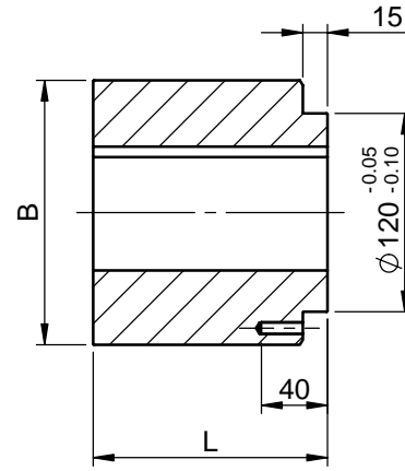
27001009700 - W-Boss/14216070G7/20/120
