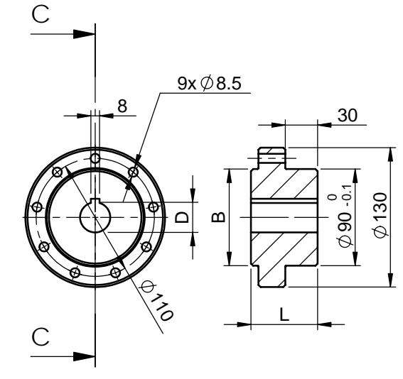
27000703300 - W-Boss/629028H7/8/90/HP
