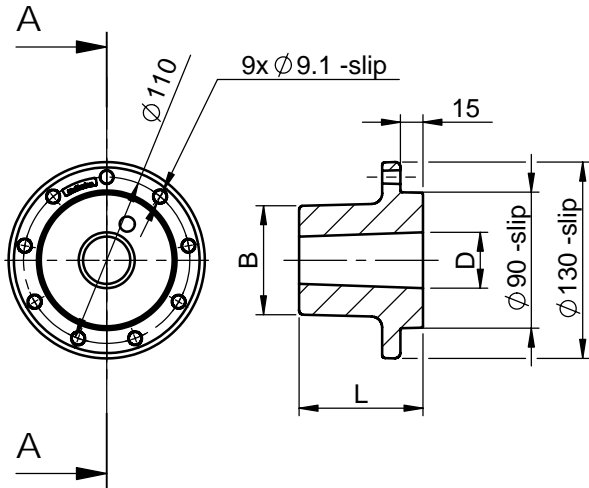
27000711606 - W-Boss/827237/90/P
