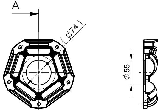
21050700103 Z-Retaining plate/5
